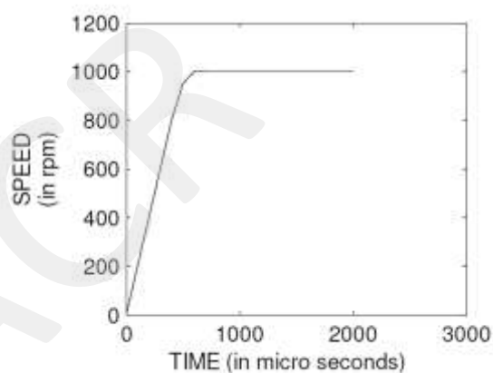
Fig.4 Speed curve attained using PSO-PID Controller.
