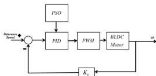
Figure 2: Block Diagram of PSO-PID Controller
