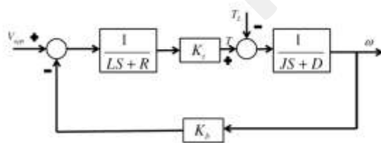
Figure 1: Block Diagram of BLDC Motor
