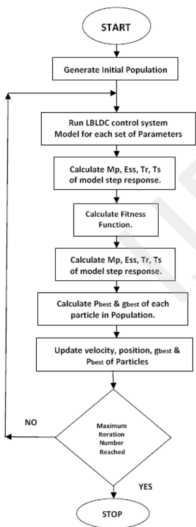
Figure 3: Flow Chart of Proposed Work
