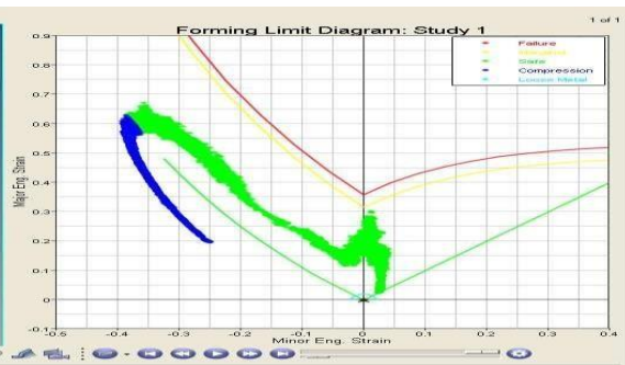
Figure 8: Formability Analysis
