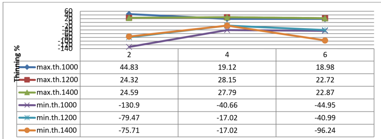
Figure 12 Effect of die entry radius on thinning % at different BHF of blank thickness 1 mm
