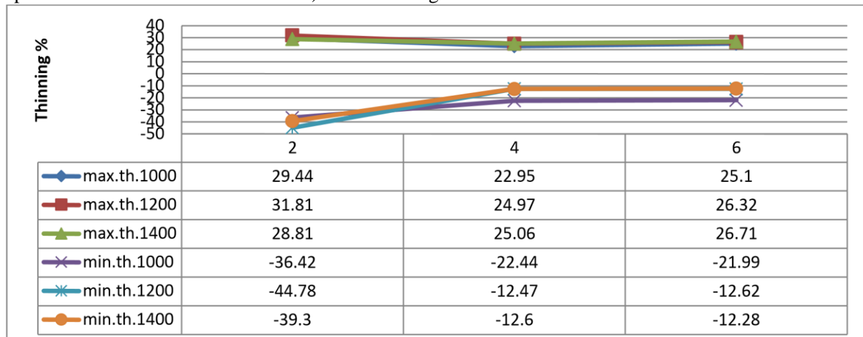
Figure 13: Effect of BHF on thinning % at different die entry radius of blank thickness 1 mm
