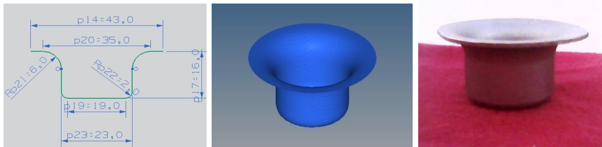
Figure 1: Component details and drawing - solid model and actual component Material
