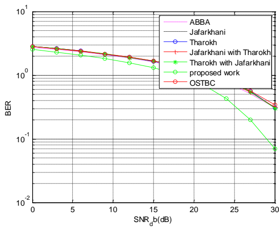
Figure 10: Variation in BER for different coding scheme for 128 PSK with ZF equalizer
