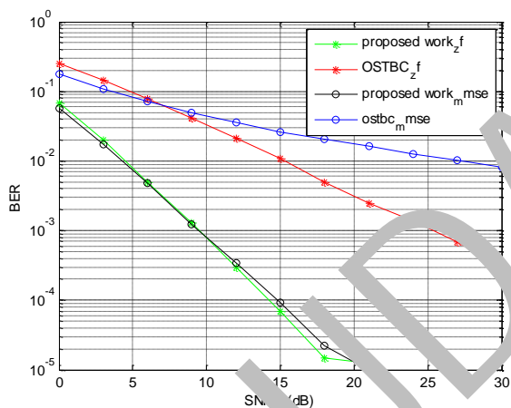
Figure 11: Variation in BER for OSTBC and proposed work with ZF and MMSE equalizer
