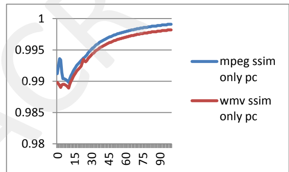
Fig 5: SSIM of real time video streaming for single accesses, compared with MPEG and WMV formats at different times
