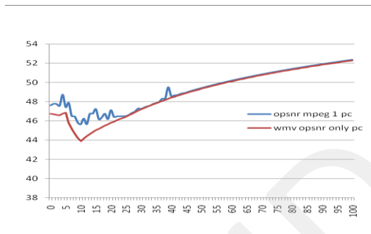
Fig 2: PSNR of real time video streaming for single accesses, compared with MPEG and WMV formats at different times
