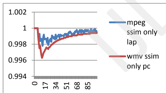
Fig 9: SSIM of real time video streaming for single accesses, compared with MPEG and WMV formats at different times
