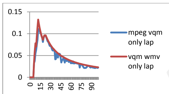
Fig 8: VQM of real time video streaming for single accesses, compared with MPEG and WMV formats at different times
