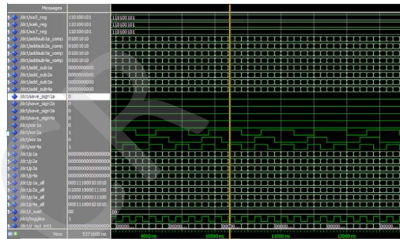
Figure8: Simulation result for 2D-DCT
