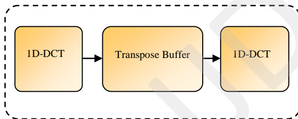
Figure3: 2-D DCT
