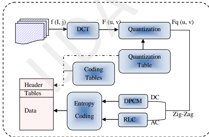
Figure2: Block diagram of Image compression
