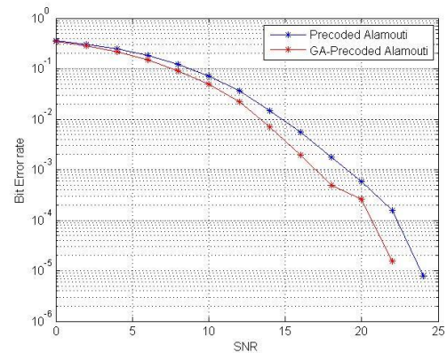
Figure 7: BER performance comparison of Precoded-Alamouti and GA optimized Precoded-Alamouti schemes in ML equalization for BPSK
