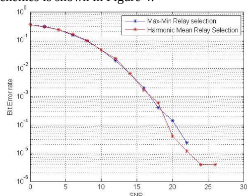
Figure 4: Comparison of BER performance for Max-Min and Harmonic-Mean relay selection schemes
