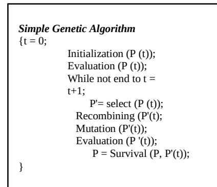
Figure 2: Steps of a simple GA
