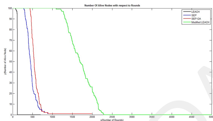
Figure4. Comparison of different protocols for Number of Alive nodes with rounds
